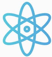
React Native
