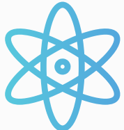
React Js
